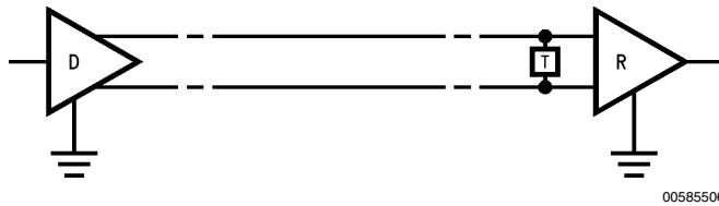
FIGURE 7. Typical TIA/EIA-422-B Point-to-Point Application
