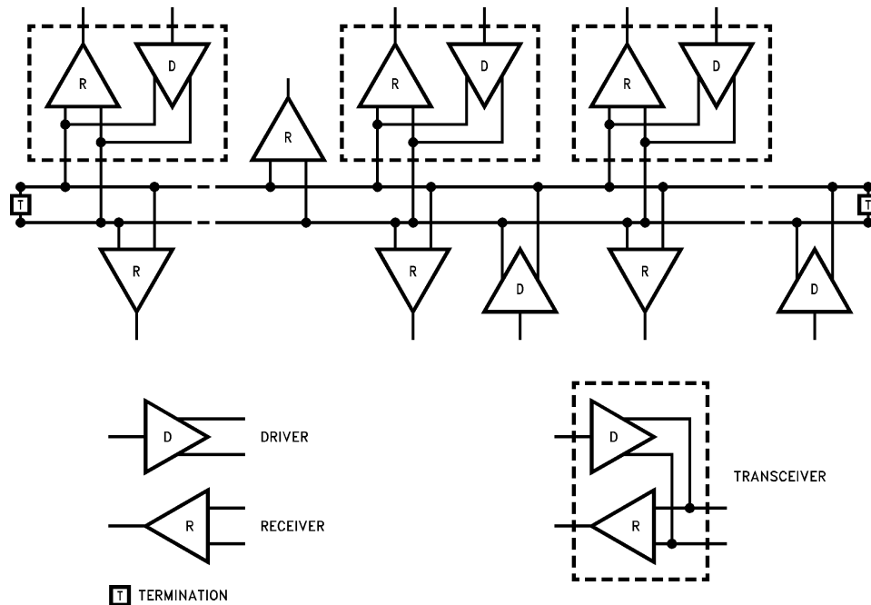
FIGURE 9. Typical TIA/EIA-485-A Application
