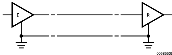
FIGURE 5. Typical TIA/EIA-562 Application
