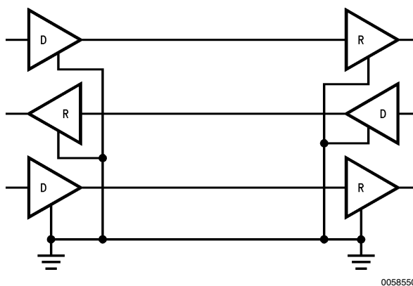
FIGURE 1. Unbalanced Data Transmission- 3 Channel, 4 Line
