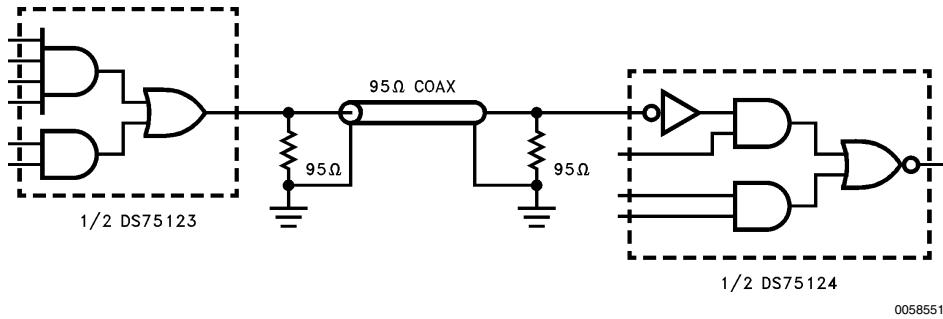
FIGURE 15. GA-22-6974-0 Typical Application
