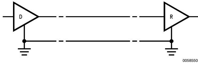
FIGURE 3. Typical TIA/EIA-232-F Application
