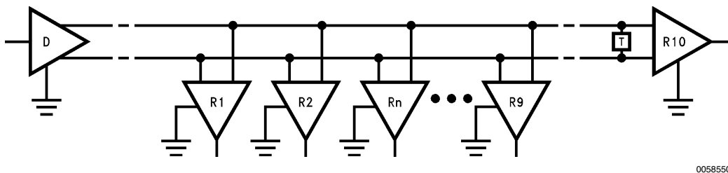
FIGURE 8. Typical TIA/EIA-422-B Multidrop Application
