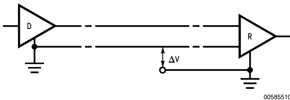
FIGURE 12. MIL STD 188-114A Unbalanced Typical Application
