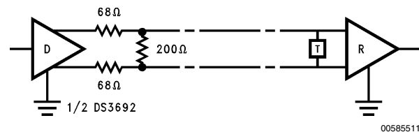
FIGURE 13. MIL STD 188-114A Balanced, Type 1 Typical Application
