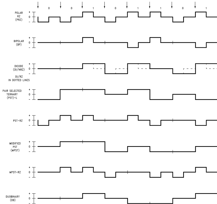
FIGURE 20. Multilevel Binary (MLB) or Pseudoternary Pulse Codes
