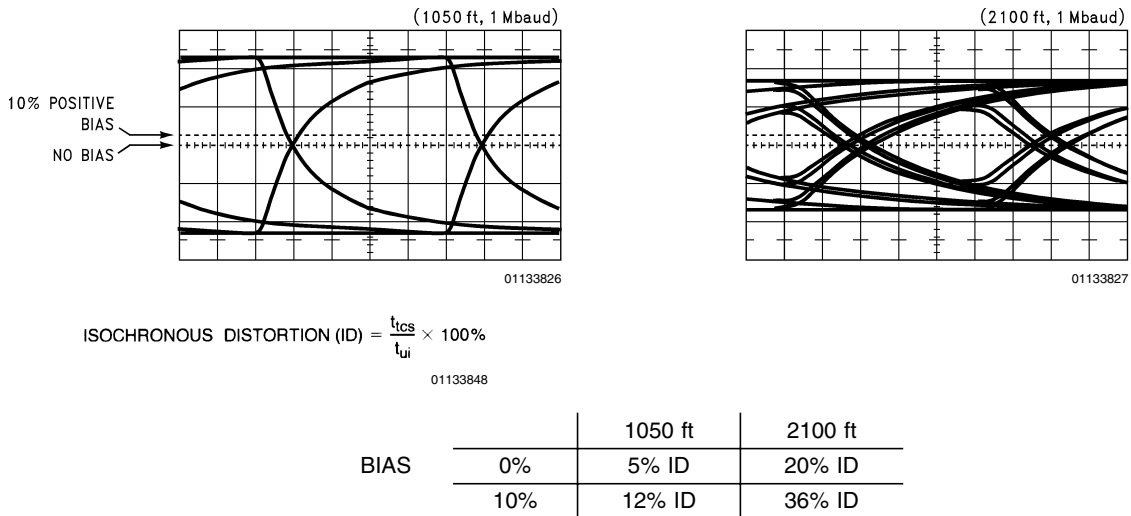
FIGURE 16. Receiver Bias Effect on Total Isochronous Distortion
