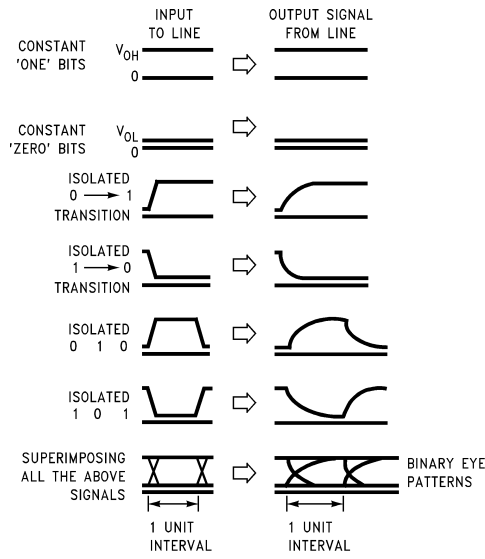
FIGURE 10. Formation of an Eye Pattern by Superposition
