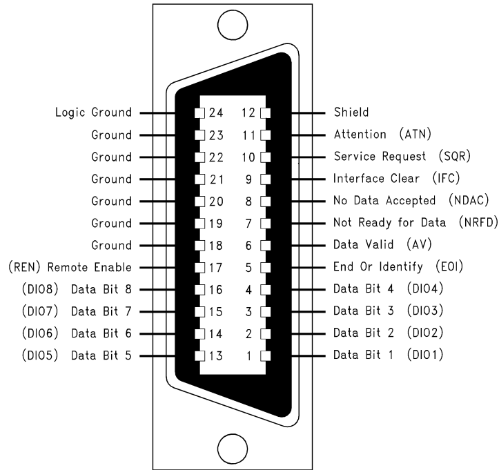
FIGURE 9. IEEE-488
