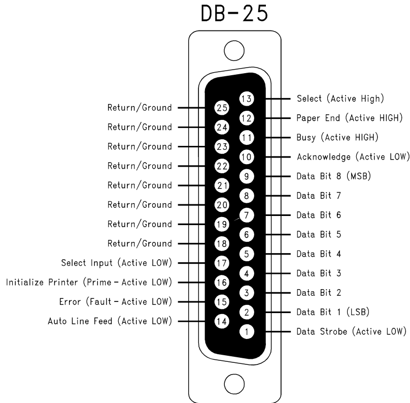
FIGURE 11. IBM PC Parallel Port
