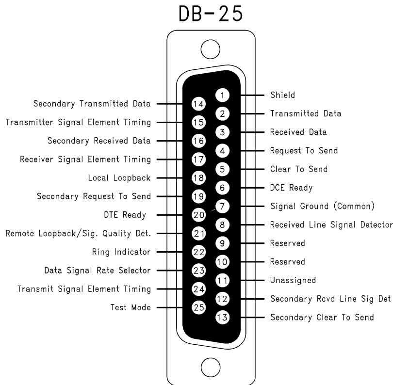
FIGURE 1. RS-232 DB-25
