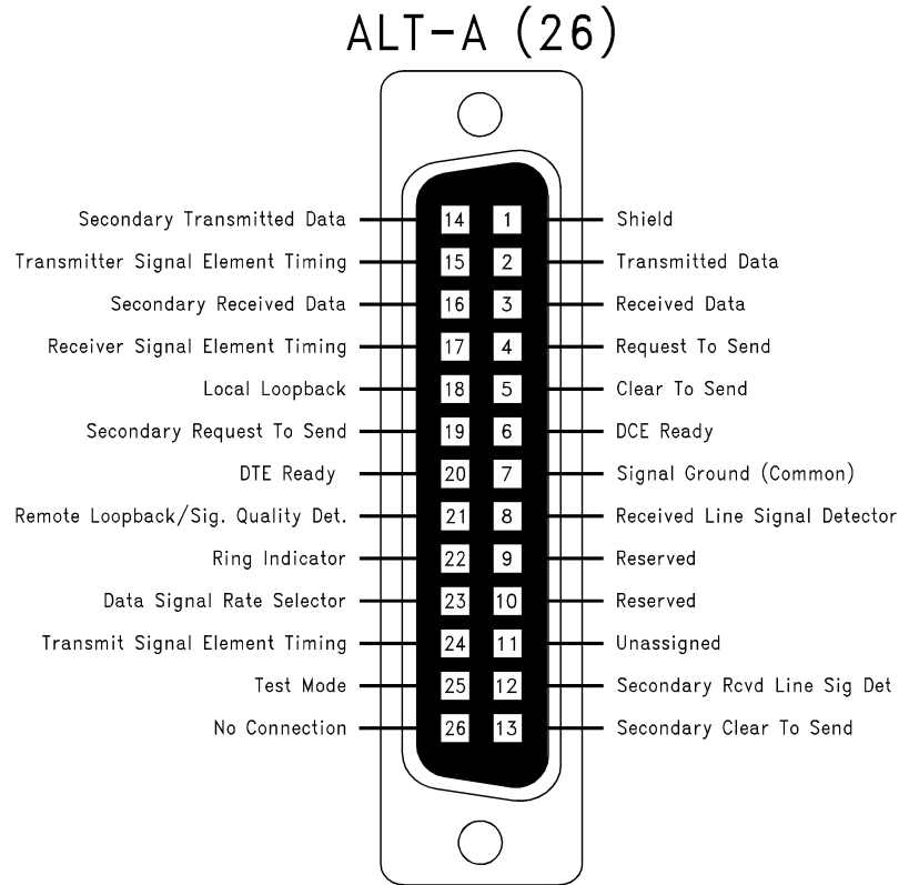
FIGURE 2. RS-232 ALT-A
