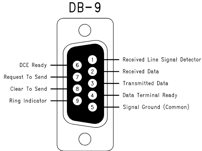
FIGURE 7. EIA/TIA-574 DB-9
