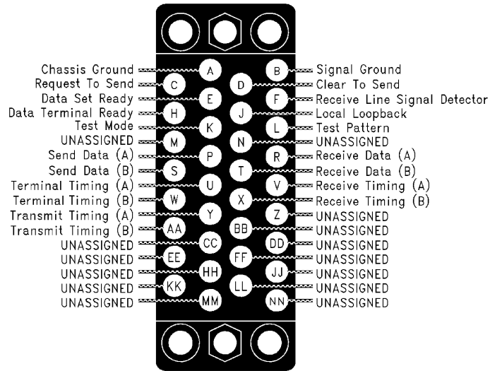
FIGURE 8. CCITT V.35
