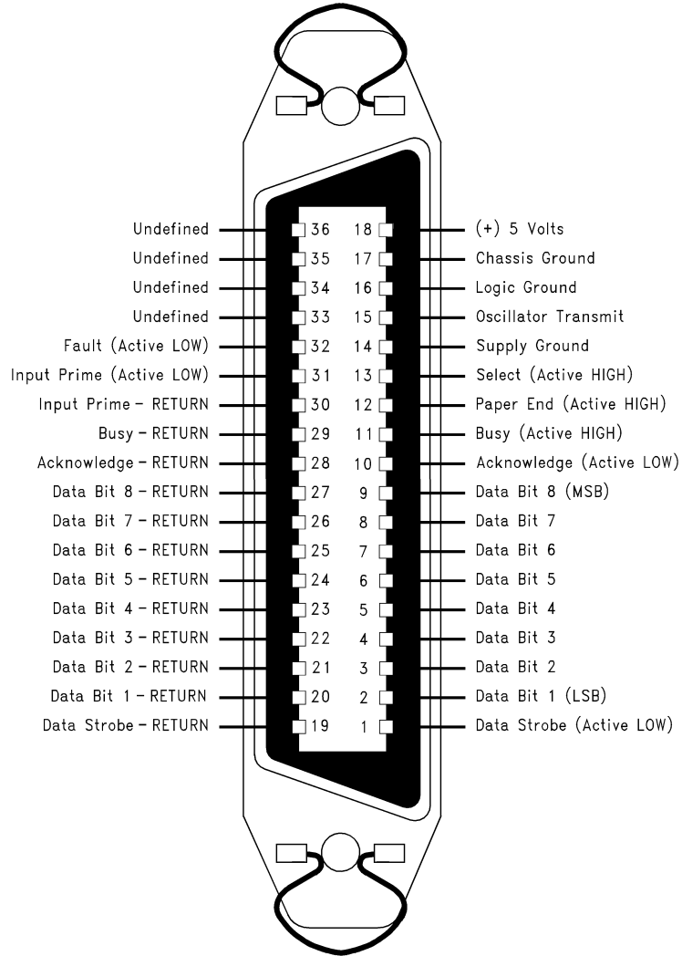
FIGURE 10. Centronics Port
