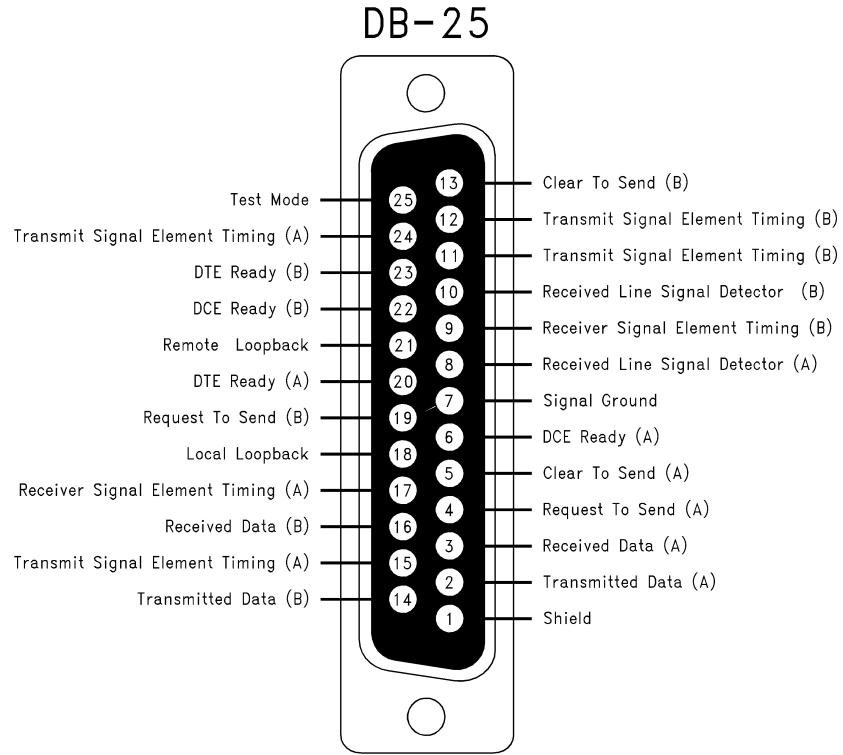
FIGURE 4. EIA-530 DB-25
